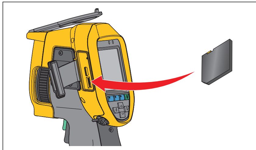
Figure 3. Micro SD Memory Card Insertion and Removal
