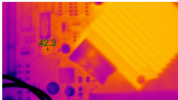
Figure 15. PCA running at 12V power supply
