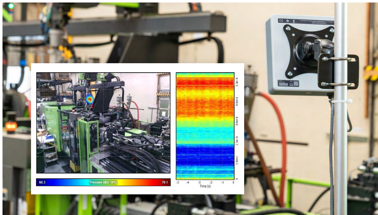
Figure 2. Condition monitoring technicians can use the new SV600 Fixed Acoustic Imager to continuously detect and locate leaks in context, while the technicians spend more time on other value-added tasks.
