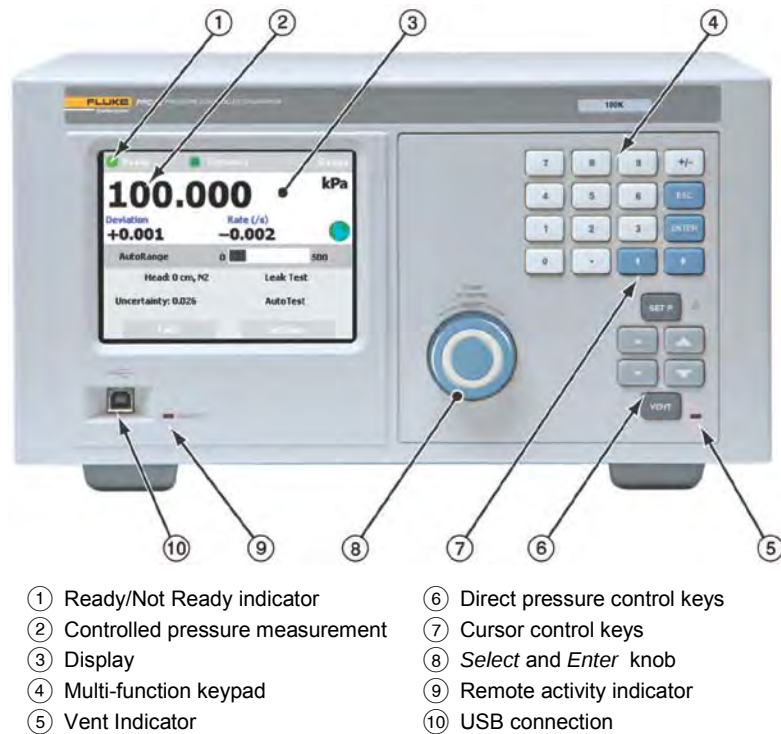
Figure 1. PPC4E front panel
