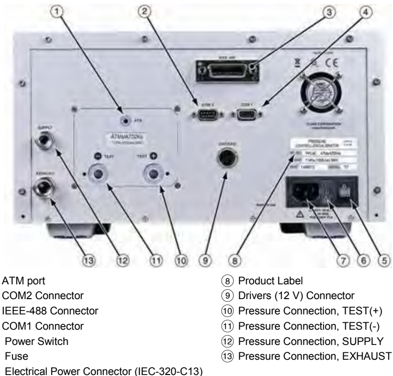
Figure 2. PPC4E rear panel
