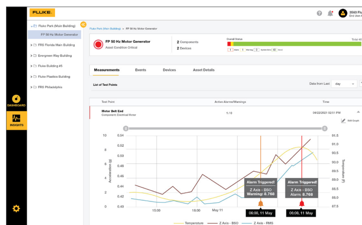
Figure 2. Configure the eMaint Condition Monitoring graph to show data from all three axes (X, Y, Z), velocity, or acceleration, and show Bearing Severity Overall trend — an exclusive 3563 sensor feature.
