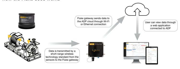
Figure 3. Data transmission sequence for the 3563 Analysis Vibration Sensor
