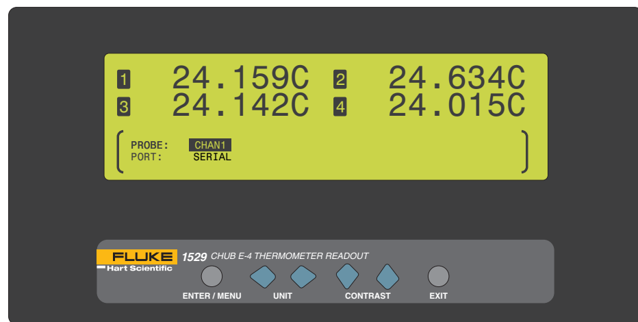
Figure 17 Print Probe
