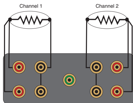
Connecting 3-wire probes
